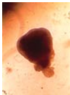
Figure 21. Embryon transparent.
